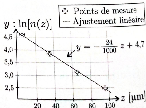
FIGURE 1 – Sédimentation de grains
