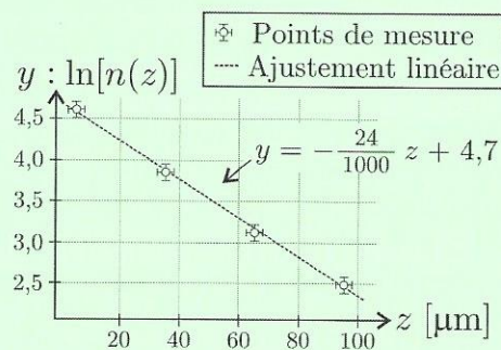
FIGURE 1 – Sédimentation de grains
