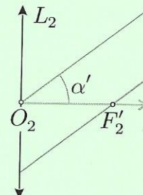
FIGURE 4 – Angle \alpha'
