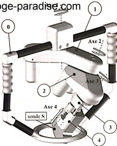
Figure 2 - Robot porte-sonde
