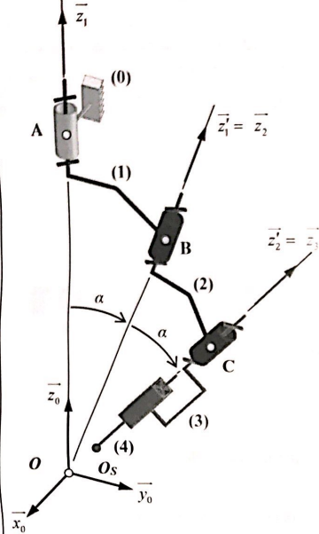
Configuration bras tendu : \theta_1 = \theta_2 = 0
