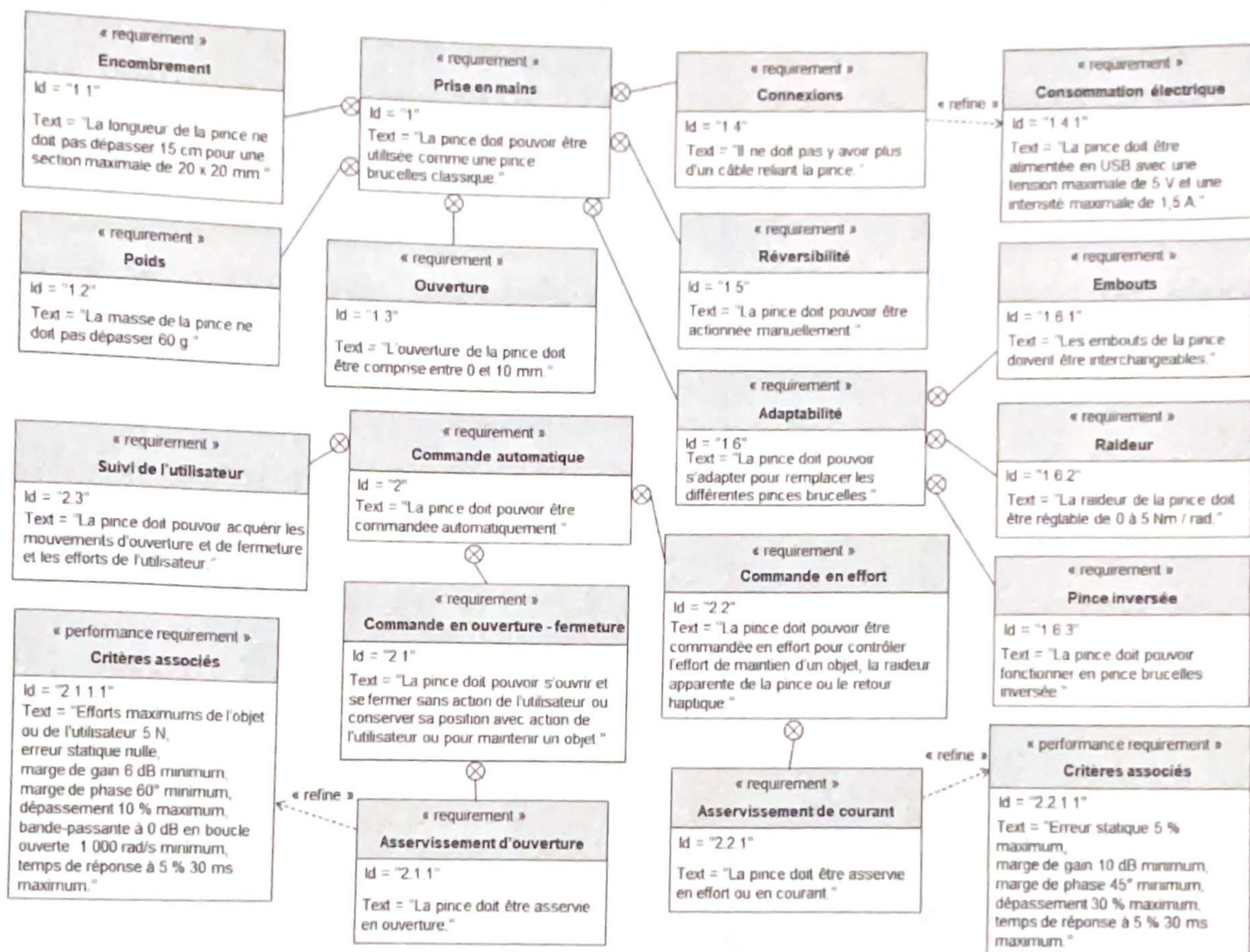
Figure 10 - Diagramme SysML partiel des exigences
