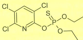
Figure 8 - Structure du chlorpyrifos
